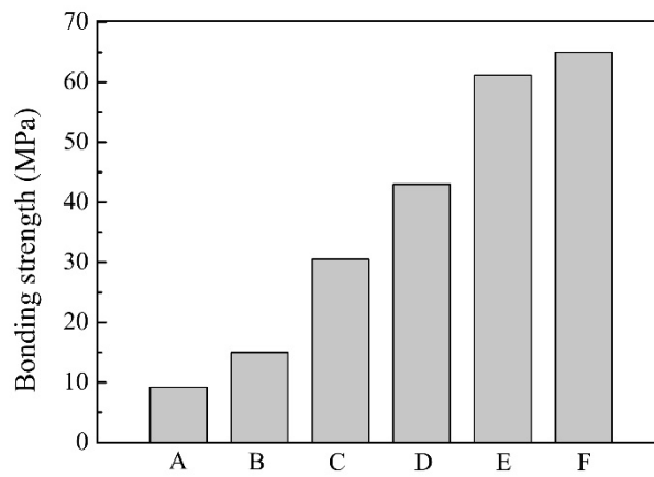
Figure 10: Bonding strength of different thermal sprayed coatings: A [52]: plasma sprayed hydroxyapatite, B [53]: plasma sprayed YSZ, C [54]: plasma sprayed Ni 20 Cr, D [55]: HVOF sprayed Fe-based amorphous composite, E [54]: plasma sprayed Ni 20 CrMo and F [56] plasma sprayed Al-Si and B 4 C composite
