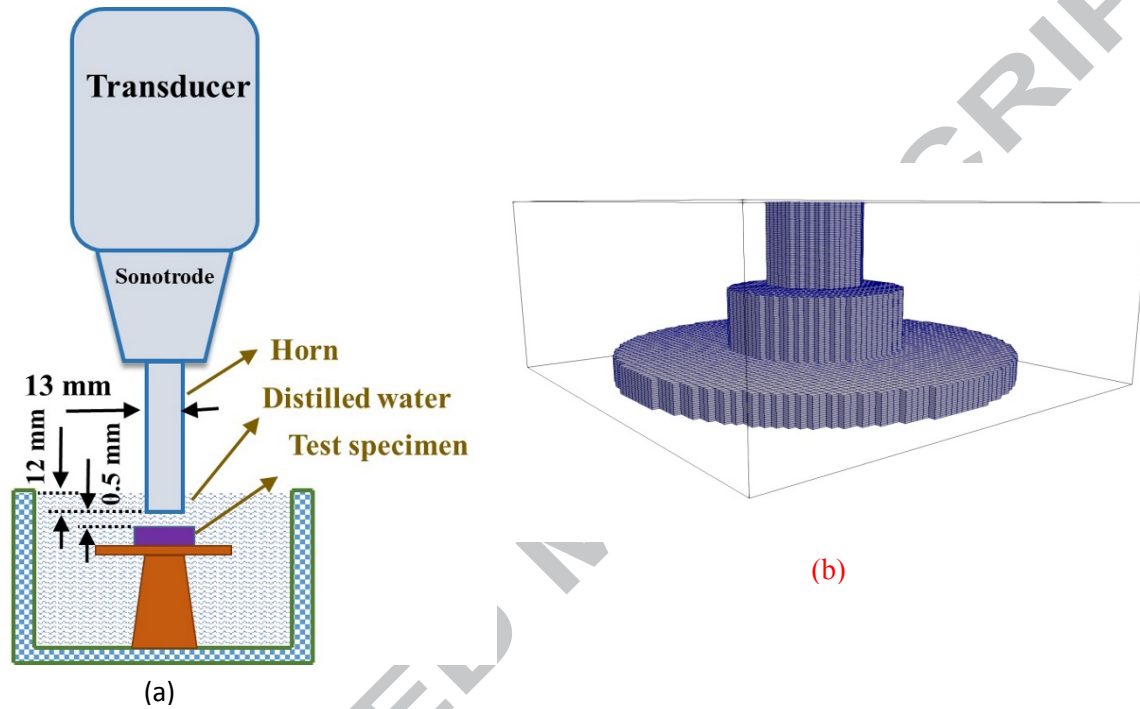
Figure 3: (a) Cavitation erosion test device (b) Castellated mesh of horn, test specimen, and supporting stand in the computational domain
